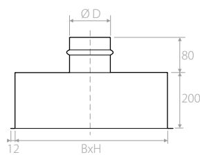
Air supply duct
