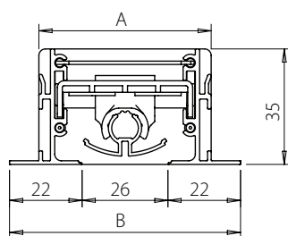
DLDT with 1 slot
