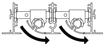
Horizontal standard throw
