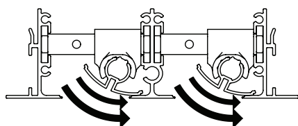
Horizontal high air flow throw
