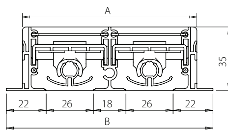
DLDT with 2 or more slot
