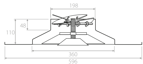
Detail of the diffuser attachment to the duct
